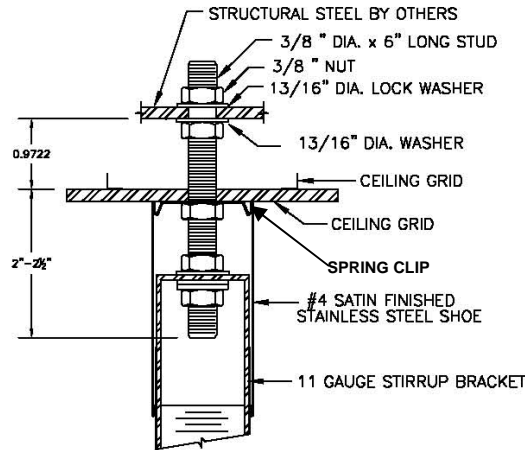
CEILING BOLT DETAIL METAL PILASTERS
